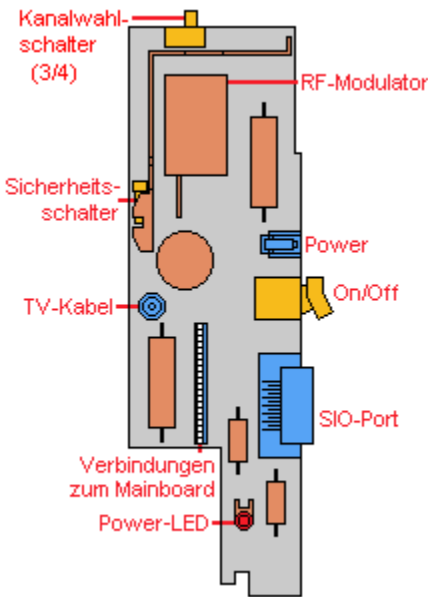
Abb. 4.8: Power-Board 400
