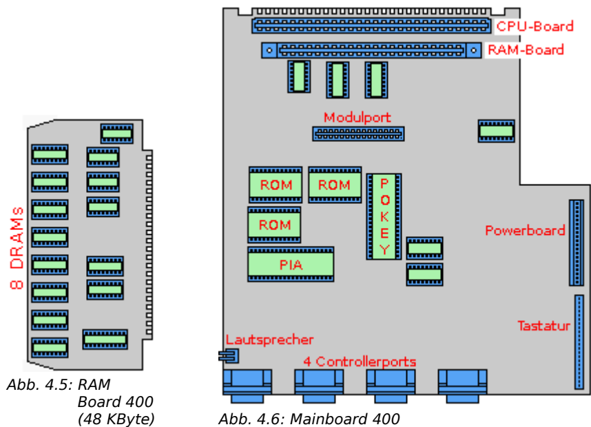
Abb. 4.6: Mainboard 400
