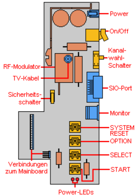
Abb. 4.15: Power-Board 800 (PAL)
